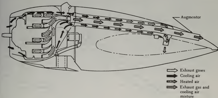
FIGURE 6-36. Augmentor.
